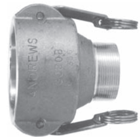
reducing female coupler x male NPT
